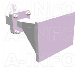
LB-62-15-C-TFSP Standard Gain Horn Antenna 12.4-18GHz 15dB Gain TNC Female
