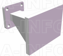
LB-62-15-ASPO Standard Gain Horn Antenna 12.4-18GHz 15dB Gain Rectangular Waveguide Interface
